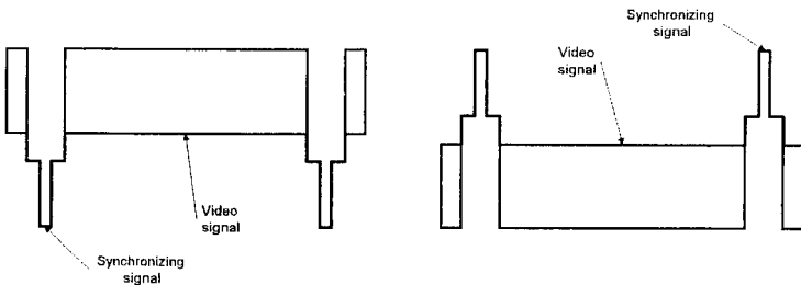
Figure 5-15 TV Signal
