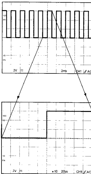
Figure 5-8 Magnified Waveform
