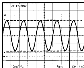
Figure 5-19: Cursor Measurement
