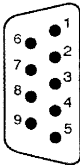
Figure 5-20. Pin assignments of the RS232 connector on the rear panel for DB-9-D
